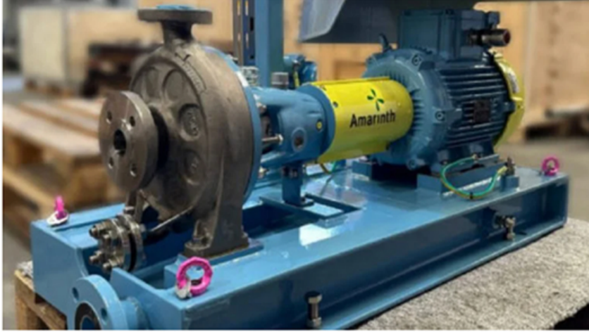
Amarinth's pump design is tailored for low net positive suction head (NPSH) duties. Credit: Amarith.
