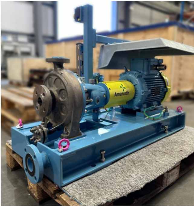
Amarinth pump nearing the end of assembly (Image source: Amarith Ltd.)
